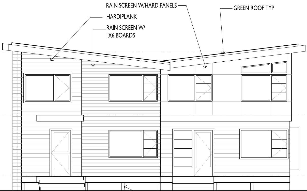
TOWNHOME - FRONT
